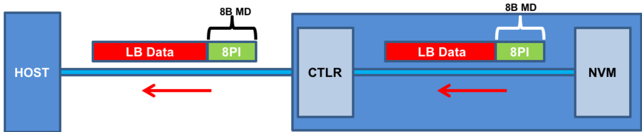
Figure 134: Read 16b Guard Command Protection Information Processing
